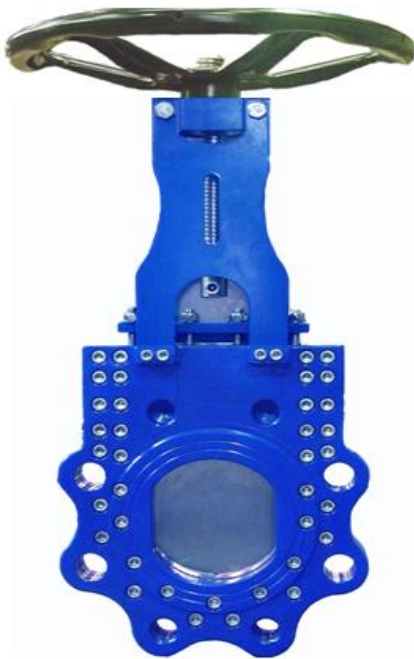
XDV-HP Bi-directional high pressure KGV, resilient (NBR) seated manual rising stem
